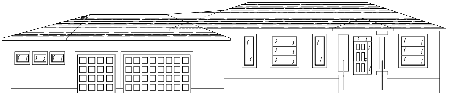
—FRONT ELEVATION—
